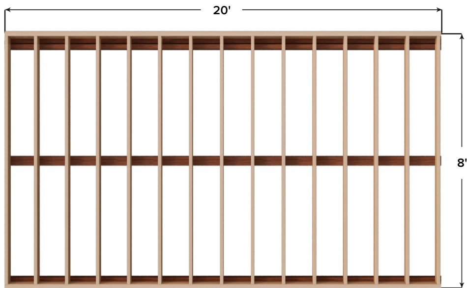
FOUNDATION BASE
