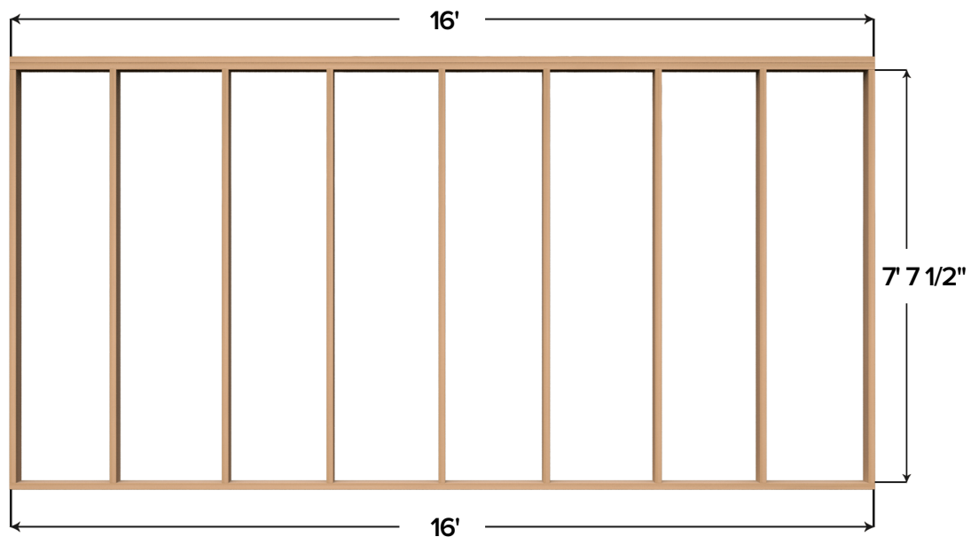
RIGHT WALL
