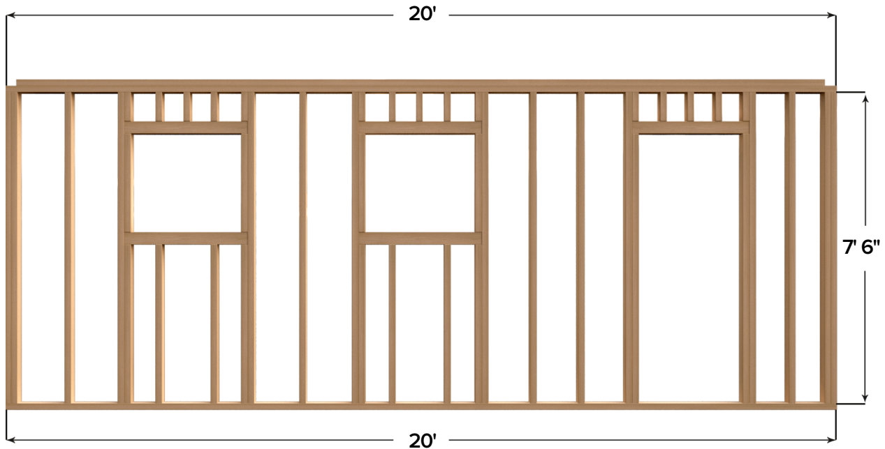
RIGHT WALL
