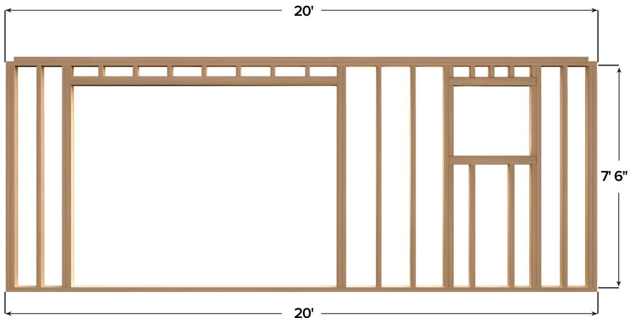
RIGHT WALL
